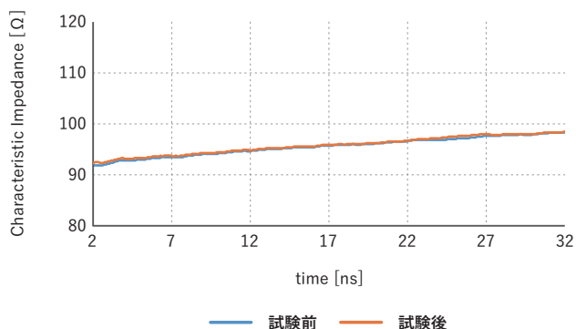
Characteristic Impedance測定結果
